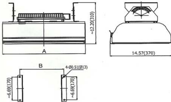
MHT-TL-100/150/200/250/300/400E
