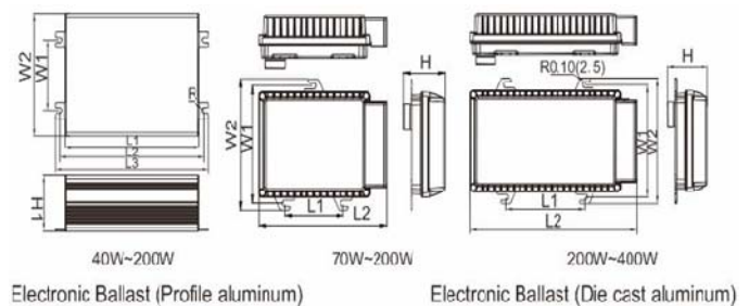
Electronic Ballast (Profile aluminum)
