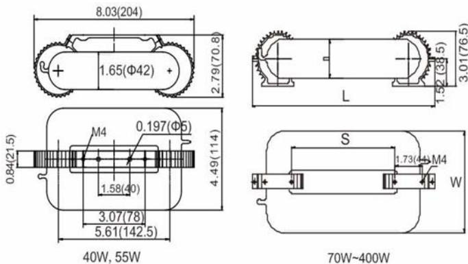
Electronic Ballast (Profile aluminum)
